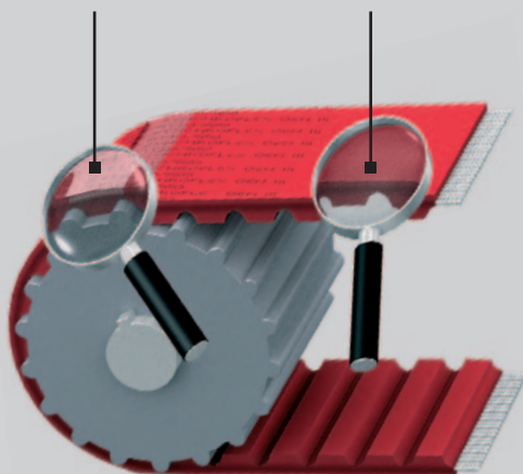
Two-filament tension member arrangement
